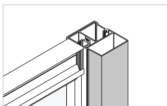
With cover strip - conceals all fixings
