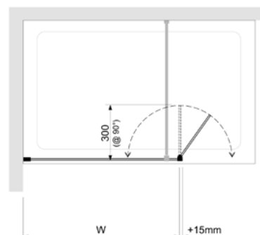
WETROOM PANEL WITH DEFLECTOR
