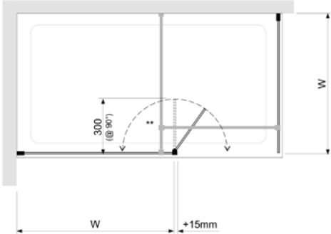
WETROOM FRONT AND SIDE PANEL WITH T BRACE AND DEFLECTOR PANEL
