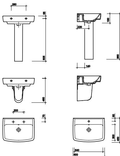
Alcona 600 x 450mm washbasin
