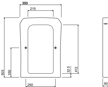
Avalon 50mm extension
