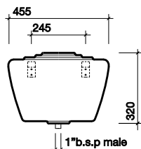
VC - 9 AND 14 LITRE CISTERNS
