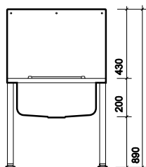
Floor standing bucket sink
