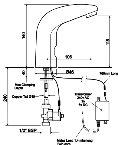
Sola infra-red tap - mains
