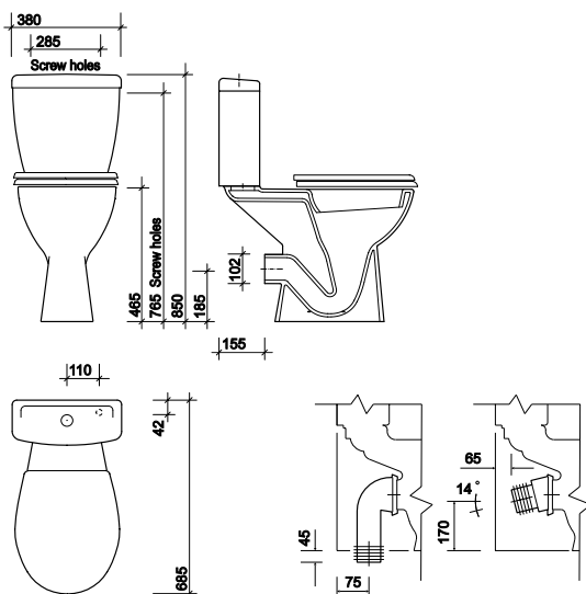
Option raised height WC suite, horizontal outlet
