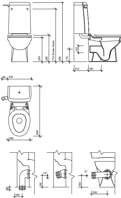
Sola school rimless 350 close coupled washdown WC suite
