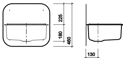
Wall-hung bucket sink
